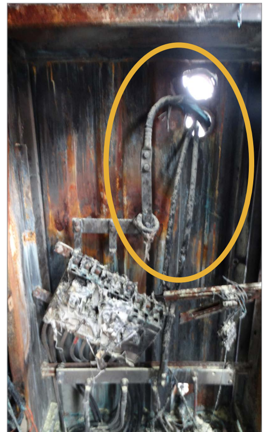
The electrical cable chafed wiring insulation in contact with the container. Picture credit Envista Forensics.
